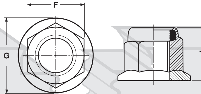
NYLON INSERT FLANGE LOCKNUTS
