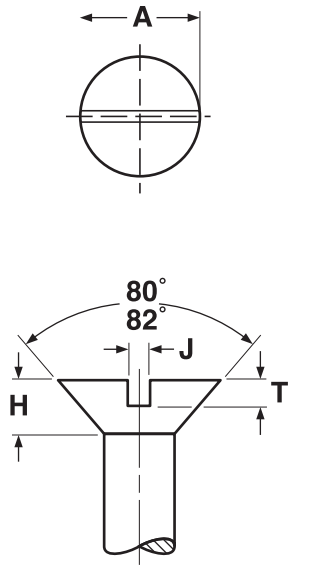
Slotted
