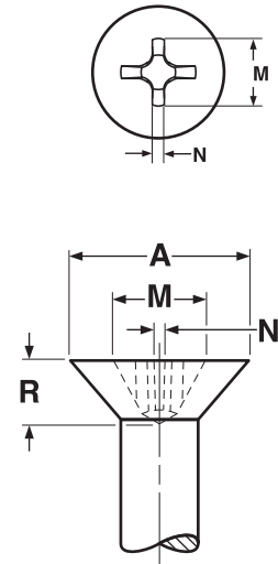
Phillips
